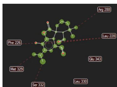
Rosmadial
