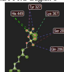
Geranyl diphosphate
