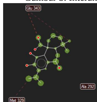
Carnosolic acid
