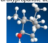
Borneol 3D
