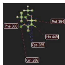
Methyl 2-[bis(2,2,2-trifluoroethoxy)phosphoryl]propanoate
